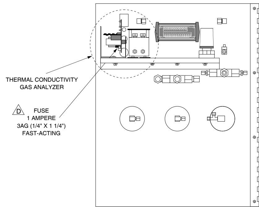
VIEW OF BACK OF INNER PANEL SHOWING ANALYZER
