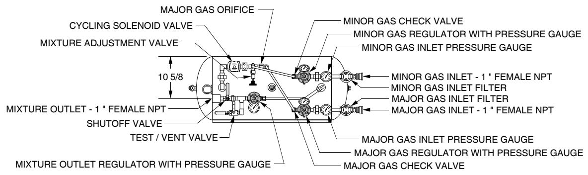
TOP VIEW (TOP REMOVED, ANALYZER AND HORN NOT SHOWN)
