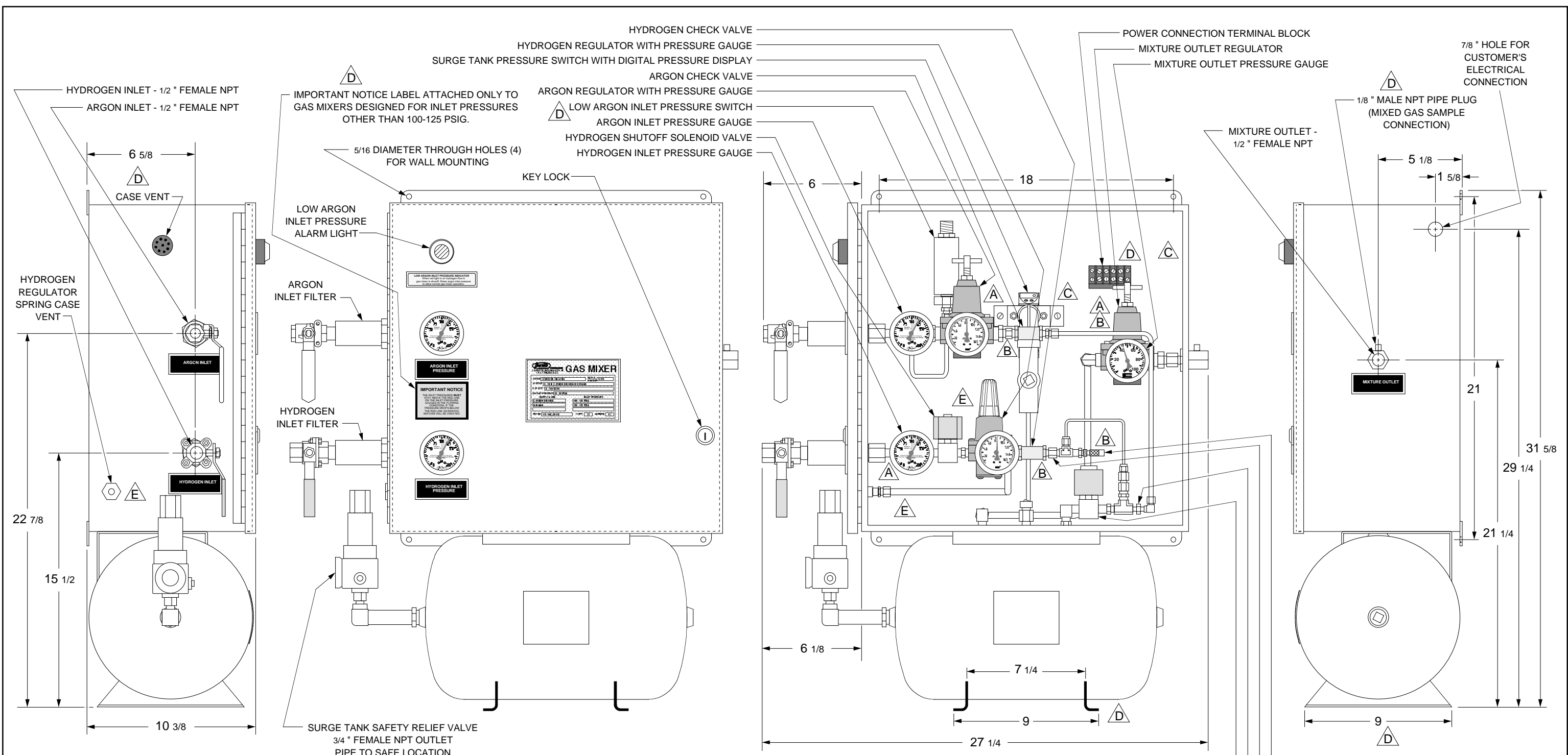
LEFT END VIEW
